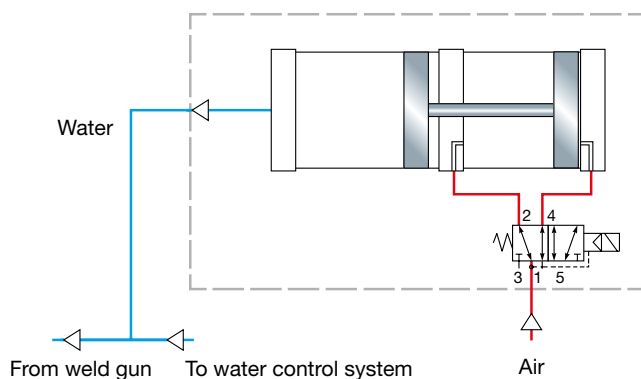
Retracted Position
