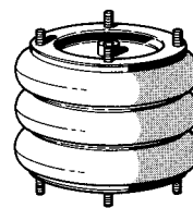
Three convolutions
