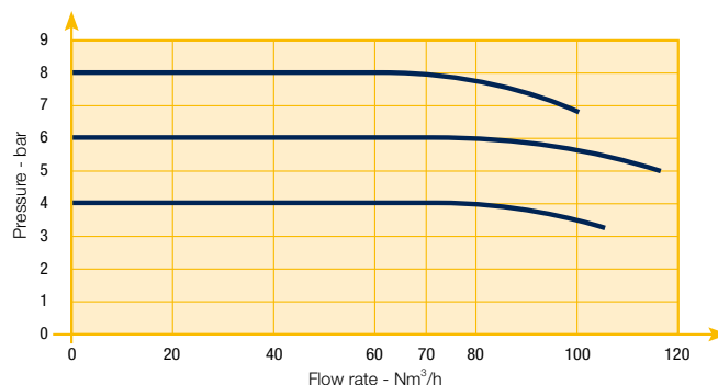
Flow Curve 1/4"
