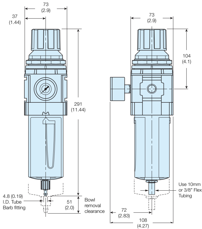
Manual Drain
