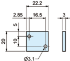
Blanking plate for pressure bar, P2LB
