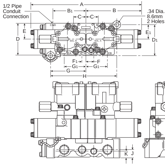
L6653 3/8" Dimensions, 3-Position, Double Solenoid
