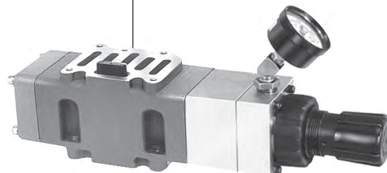
Regulator Assembly
