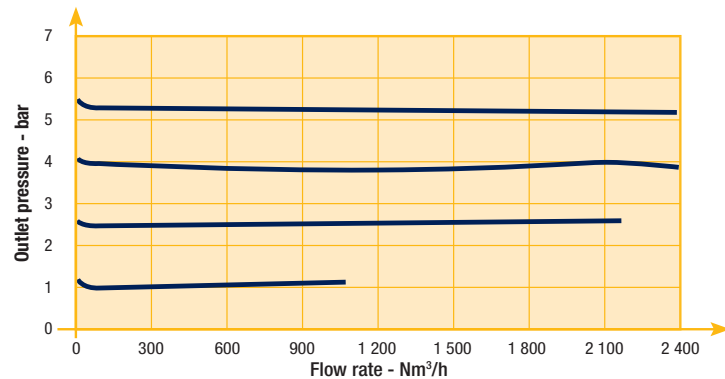
Flow Curve 2"
