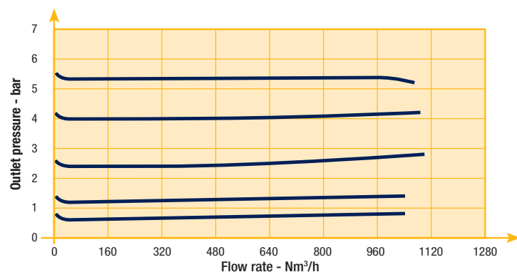
Flow Curve 2"
