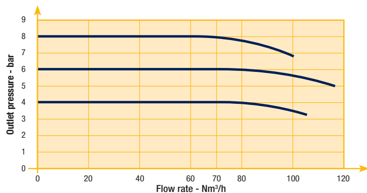
Flow Curve 1/4"
