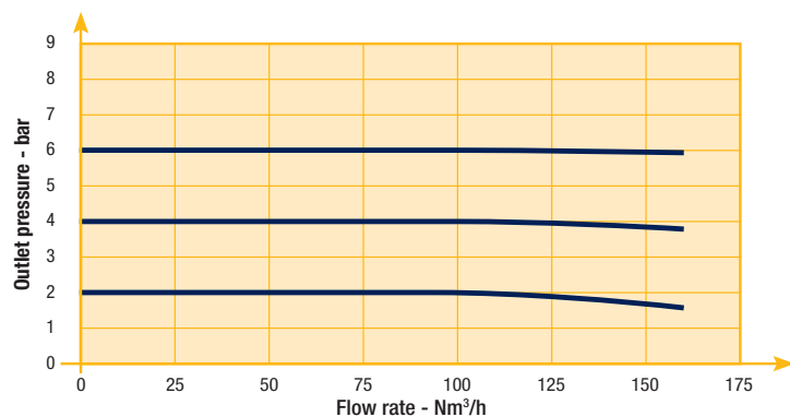
Flow Curve 1/2"
